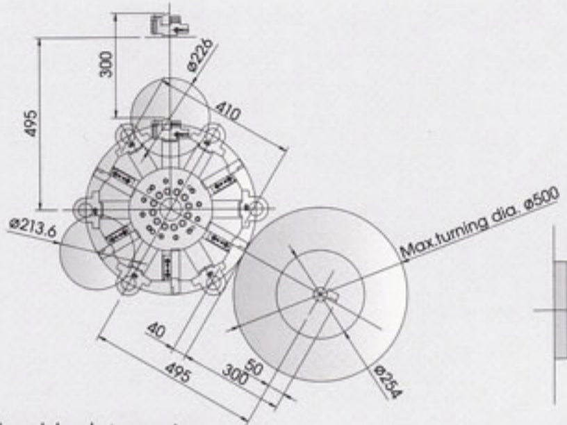
12-Station block turret
